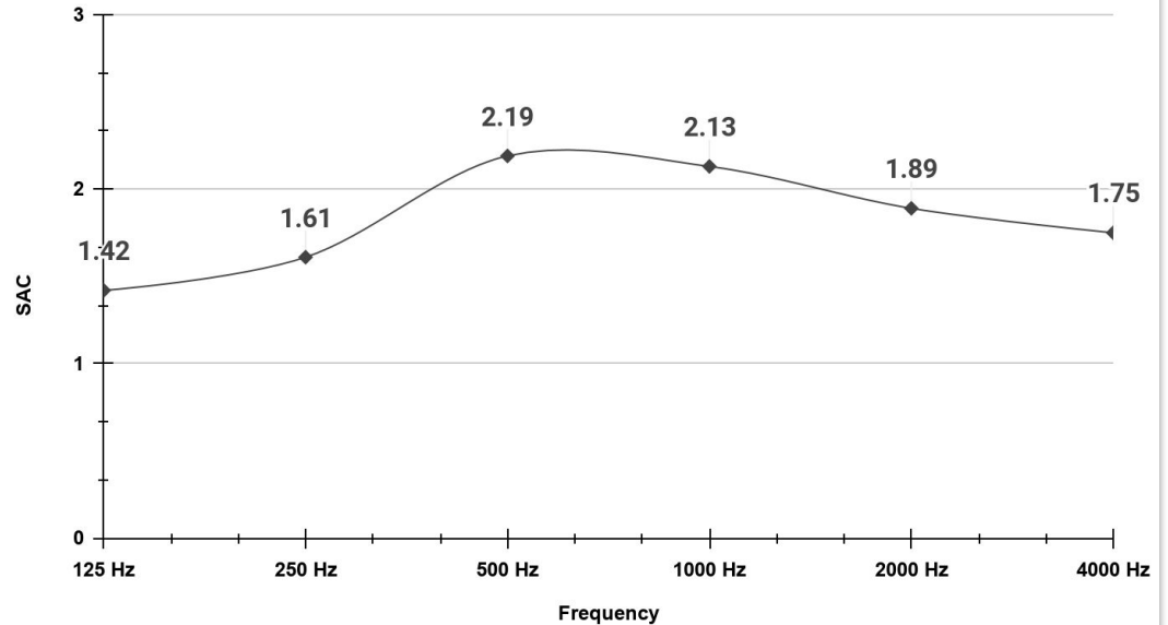
EconoMegaWedge™ Diffuser NRC 1.95
