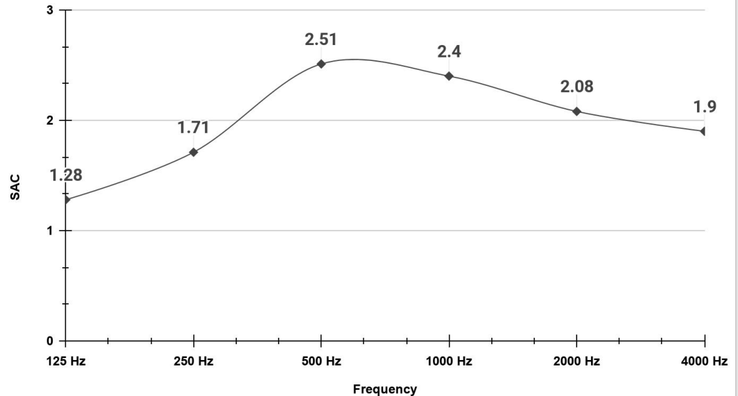
EconoMaxWedge™ NRC 2.20
